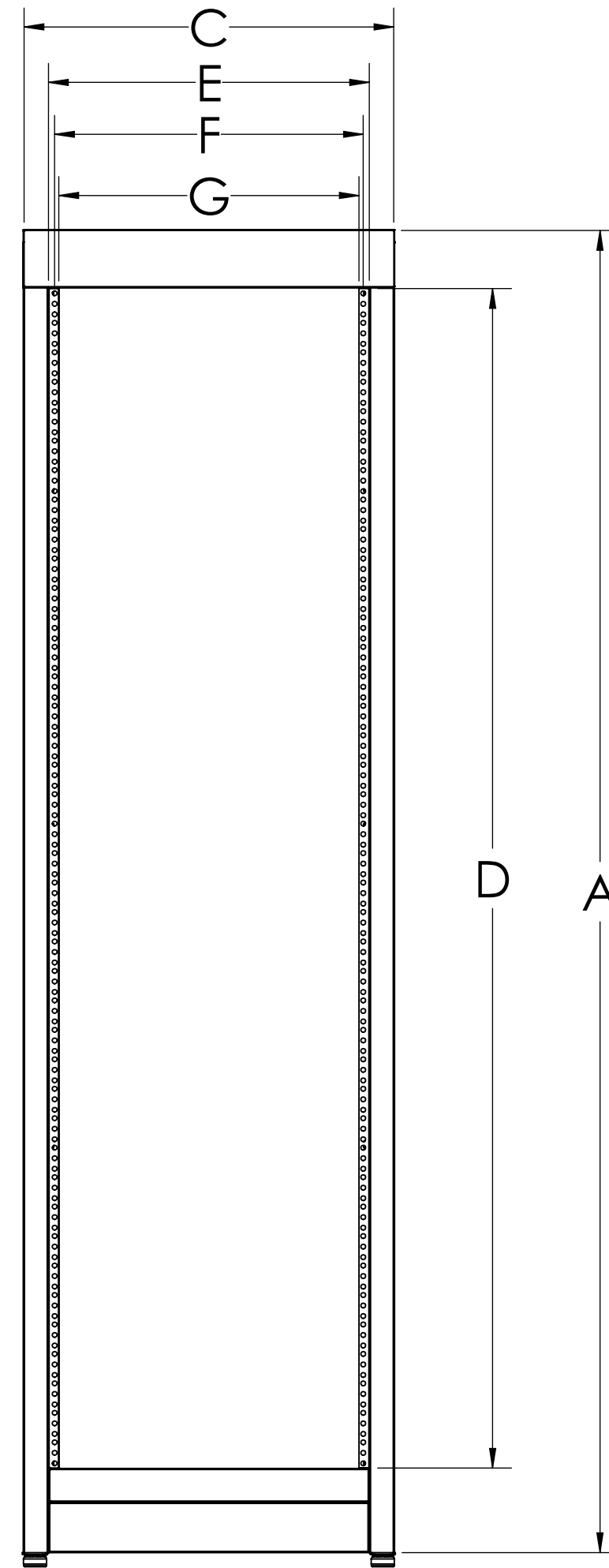
FRONT VIEW
