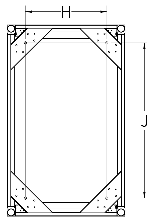
BOTTOM VIEW
